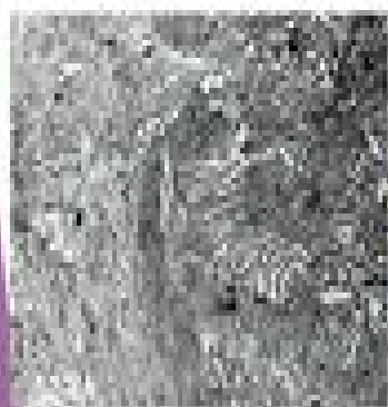
CEMENTITA
